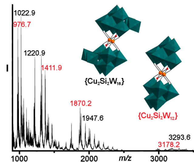
Figure 2. ESI-MS of THA[ \text{Cu}_2(\beta\text{-SiW}_8\text{O}_{31})_2 ] showing the most intense envelopes for the intact \{\text{Cu}_2\text{Si}_2\text{W}_{16}\} (highlighted in black) and fragmented \{\text{Cu}_2\text{Si}_2\text{W}_{12}\} species (highlighted in red).
